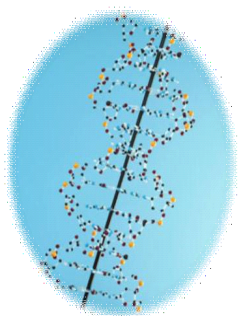
Genomics
